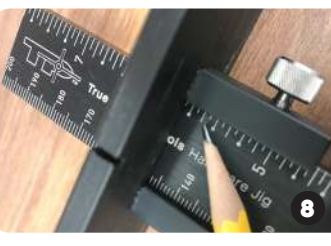
8 Set the Large Stop and tighten at desired location
