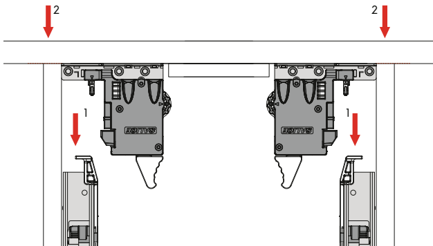
Drawer Assembly
